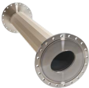
Vacuum chamber made of FRIALIT F99.7, metal-to-ceramic bond (length 1350 mm, diameter 320 mm)
