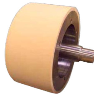
Ceramic roller body made of FRIALIT F99.7 (outer diameter 250 mm), metal-to-ceramic bond
