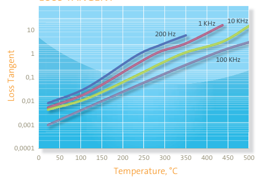
LOSS TANGENT
